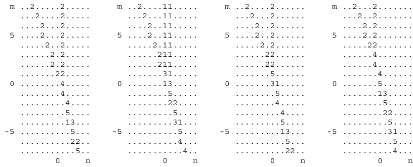
Figure 3. A (2, 1)-resonant soliton solution (i.e., a Y-junction) for the ultradiscrete 2DTL equation (6.9), with P_1 = -5, P_2 = 1, P_3 = 4, r = 3, s = 1, A_1 - A_3 = 1, A_2 - A_3 = 1 . From left to right, the four plots represent the solution respectively at l = 0, l = 2, l = 4 and l = 6 . The dots indicate zero values of v_{l,m,n} .
