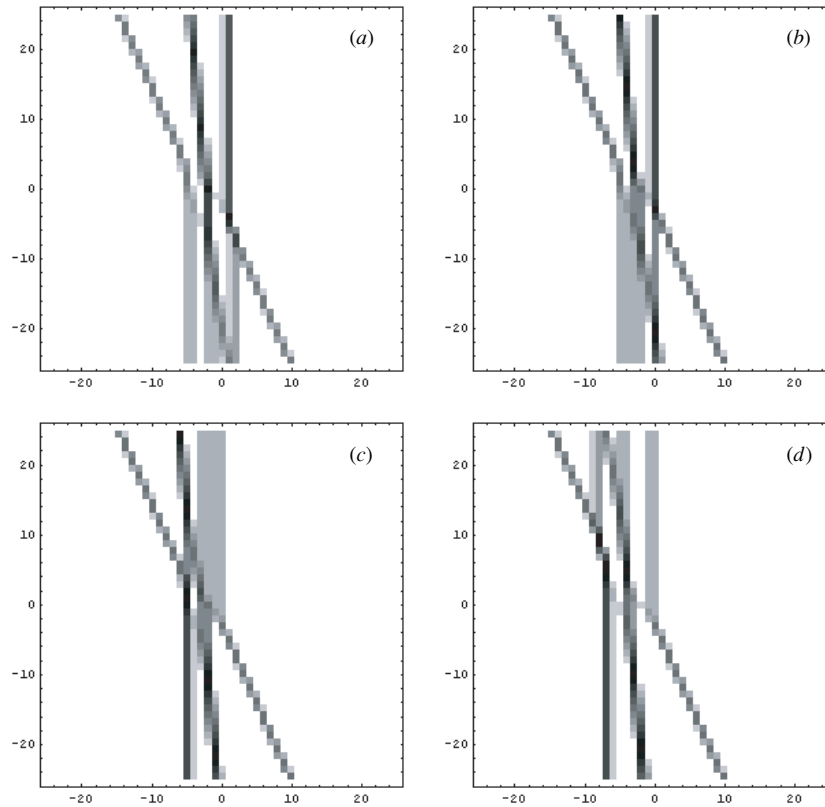
Figure 6. Snapshots illustrating the temporal evolution of a (3,3) -resonant soliton solution for equation (6.9), with P_1 = -10, P_2 = -7, P_3 = -5, P_4 = -1, P_5 = 4, P_6 = 5, r = 7, s = 4, A_1 = -8, A_2 = -6, A_3 = 0, A_4 = 2, A_5 = 4, A_6 = 7 : (a) l = -15 , (b) l = -10 , (c) l = 0 , (d) l = 10 .
