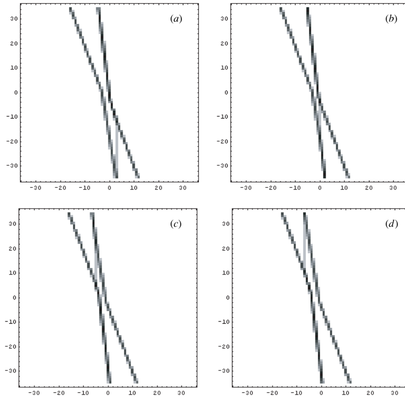
Figure 5. Snapshots illustrating the temporal evolution of a (2, 2)-resonant soliton solution for equation (6.9), with P_1 = -7, P_2 = -5, P_3 = 1, P_4 = 3, r = 4, s = 2, A_1 = -10, A_2 = -6, A_3 = 0, A_4 = 2 : (a) l = -12 ; (b) l = -7 ; (c) l = 4 ; (d) l = 7 . As in figures 3 and 4, the horizontal axis is n and the vertical axis is m . Since the interaction extends over a wider range of values of m and n , the solution is now plotted in greyscale, in a similar way as in figures 1 and 2; the values of v_{l,m,n} however are still discrete, as in figures 3 and 4.
