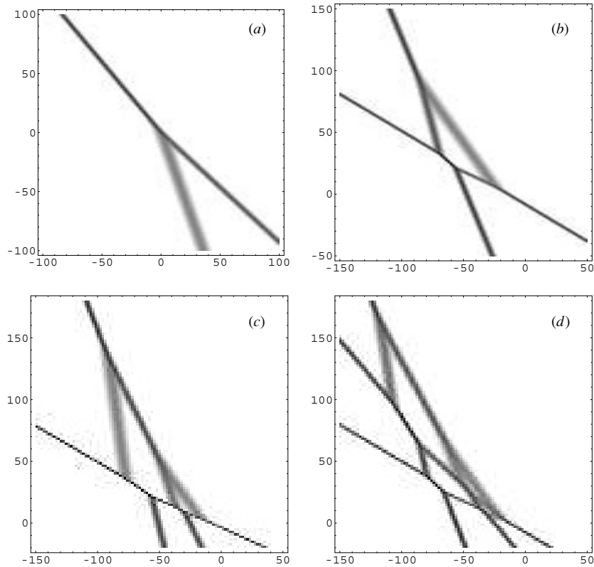
Figure 1. Resonant solutions of the two-dimensional Toda lattice: (a) (2, 1)-soliton solution (i.e., a Y-junction) at t = 0 , with N = 1 , M = 3 , p_1 = 1/4 , p_2 = 1/2 , p_3 = 2 ; (b) (2, 2)-soliton solution at t = 14 , with N = 2 , M = 4 , p_1 = 1/8 , p_2 = 1/2 , p_3 = 1 and p_4 = 4 ; (c) (3, 2)-soliton solution at t = 10 , with N = 2 , M = 5 , p_1 = 1/10 , p_2 = 1/5 , p_3 = 1/2 , p_4 = 1 and p_5 = 6 ; (d) (3, 3)-soliton solution at t = 14 , with N = 3 , M = 6 , p_1 = 1/10 , p_2 = 1/4 , p_3 = 1/2 and p_4 = 1 , p_5 = 2 , p_6 = 4 . In all cases the horizontal axis is n and the vertical axis is x , and each figure is a plot of q(n, x, t) in logarithmic greyscale. Note that the values of n in the horizontal axis are discrete.
