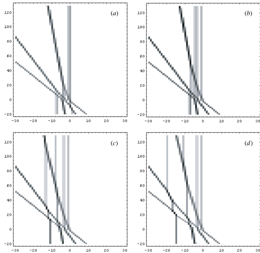
Figure 7. Snapshots illustrating the temporal evolution of a (4, 4)-resonant soliton solution for equation (6.9), with P_1 = -15 , P_2 = -12 , P_3 = -9 , P_4 = -3 , P_5 = 1 , P_6 = 1 , P_7 = 4 , P_8 = 7 , r = 7 , s = 4 , A_1 = -8 , A_2 = -6 , A_3 = 0 , A_4 = 2 , A_5 = 4 , A_6 = 7 , A_7 = 8 , A_8 = 10 : (a) l = -10 , (b) l = 0 , (c) l = 10 , (d) l = 20 .
