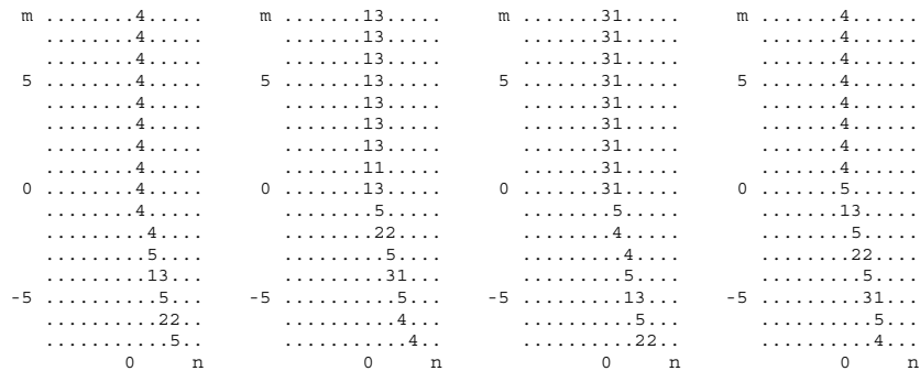
Figure 4. An L-shape (2, 1)-resonant soliton solution for equation (6.9), with P_1 = -5, P_2 = -1, P_3 = 4, r = 3, s = 1, A_1 - A_3 = 1, A_2 - A_3 = 1 . From left to right, the four plots represent the solution respectively at l = 0, l = 2, l = 4 and l = 6 .
